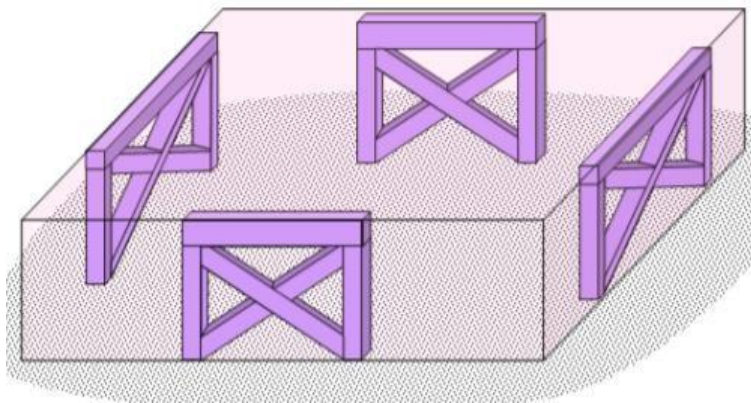
Cross-braced frames
